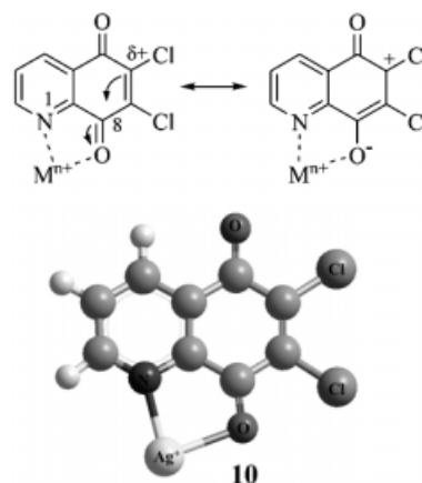
Figure 2. Metal ion coordination to 6,7-dichloroquinoline-5,8-dione ( 2 ) and the minimised structure of silver complex 10 .
