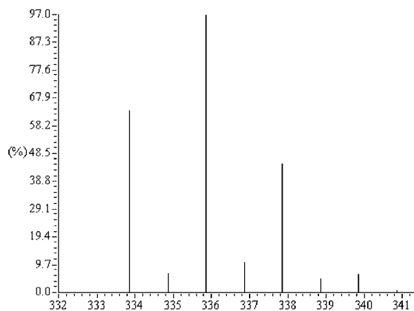
Figure 3. Experimental (left) and simulated (right) ESI(+) mass spectra for the silver complex 10 , showing the cluster with the most intense signal at m/z = 336 [C 9 H 3 AgCl 2 NO 2 + ].
