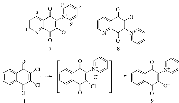
Figure 1. Structures of by-products 7–9. Adopted numbering is for convenience.
