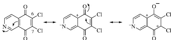
Figure 5. Resonance forms for 6,7-dichloroisoquinoline-5,8-dione ( 13 ).
