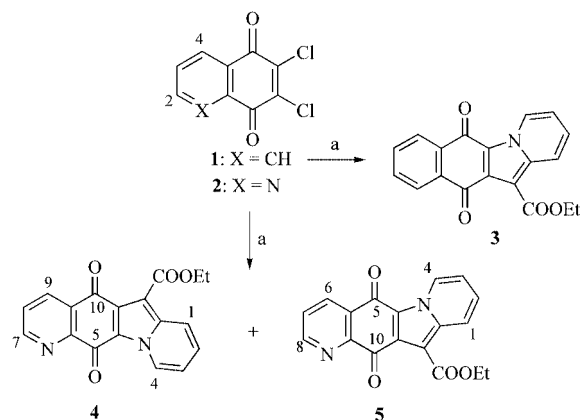
Scheme 1. Sequence for the cyclisation. Reagents: a) pyridine, ethyl acetoacetate under different conditions.
