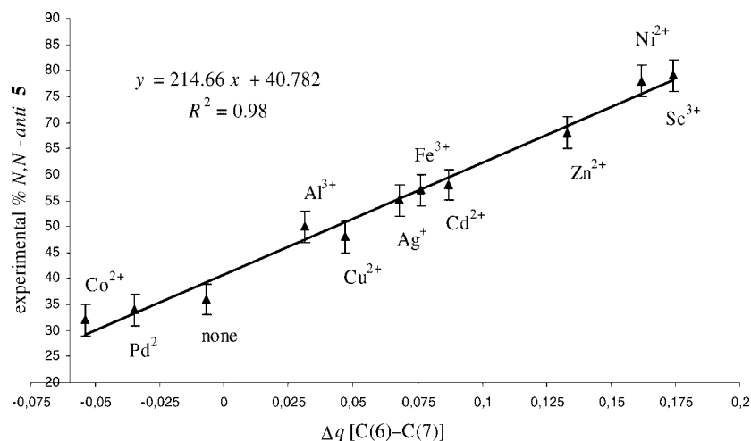
Figure 4. Linear correlation of the experimental amount of N,N -anti 5 as a function of the difference between the calculated charges at C-6 and C-7 for the regioselective one-pot synthesis in the presence of metal ions.
