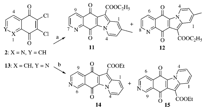
Scheme 4. Synthesis of the methyl-substituted regioisomers 11/12 and of isoquinoline-like regioisomers 14/15 . Reagents: a) 4-methylpyridine, ethyl acetoacetate under different conditions; b) pyridine, ethyl acetoacetate under different conditions.
