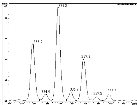
Figure 3. Experimental (left) and simulated (right) ESI(+) mass spectra for the silver complex 10 , showing the cluster with the most intense signal at m/z = 336 [C 9 H 3 AgCl 2 NO 2 + ].
