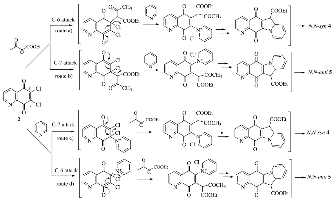
Scheme 3. Possible routes to products 4 and 5 .
