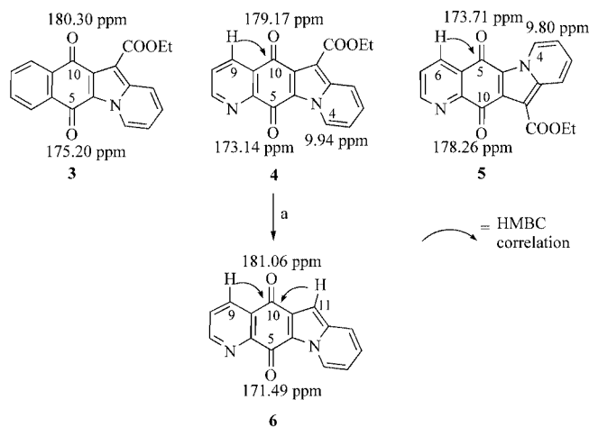
Scheme 2. Structural assignments of the N,N - syn and N,N - anti regioisomers.
